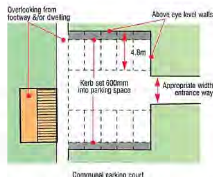
Alternative ways of accommodating parking spaces between or within buildings facing Road Types 3 - 6
