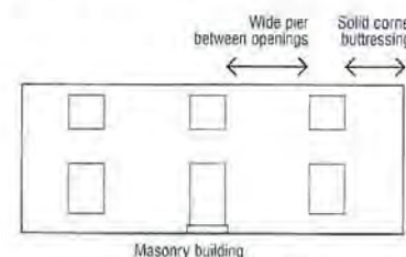
Masonry building
