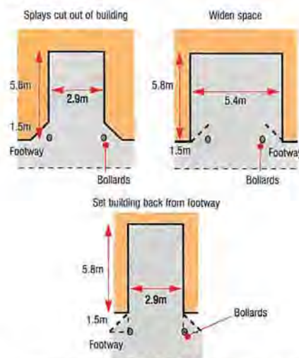
Alternative ways of accommodating parking spaces between or within buildings facing Road Types 3 - 6
